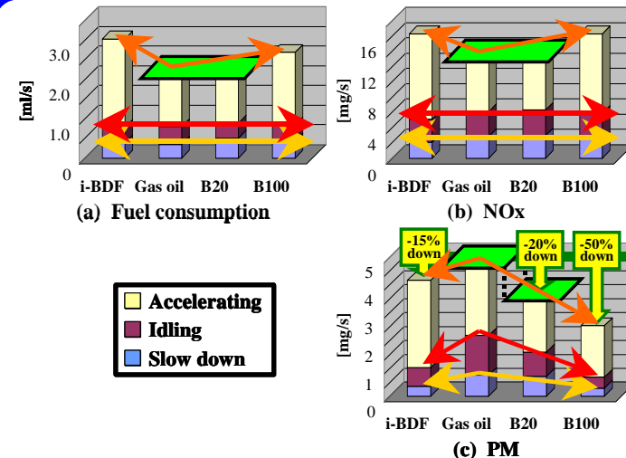
Influence of 3-mode drives at intersection
