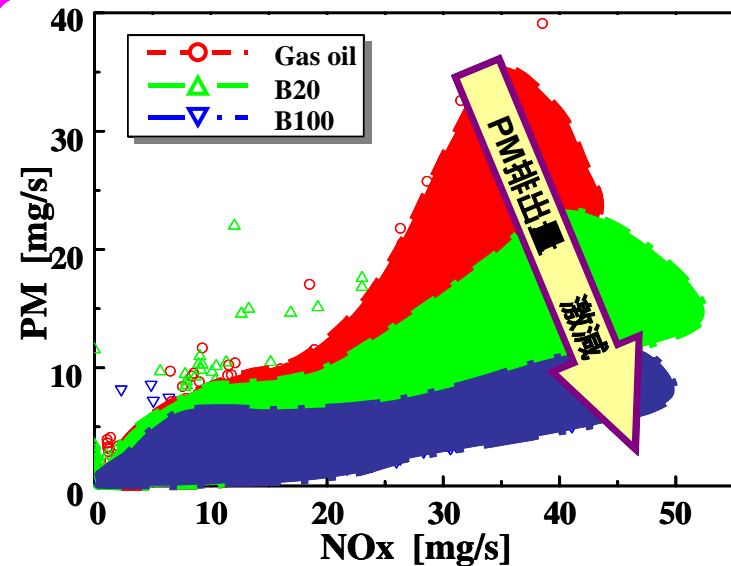
Correlation between NOx and PM emissions
